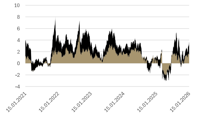
Z-Score (XBANK) — Z-Score (XUSIN)
